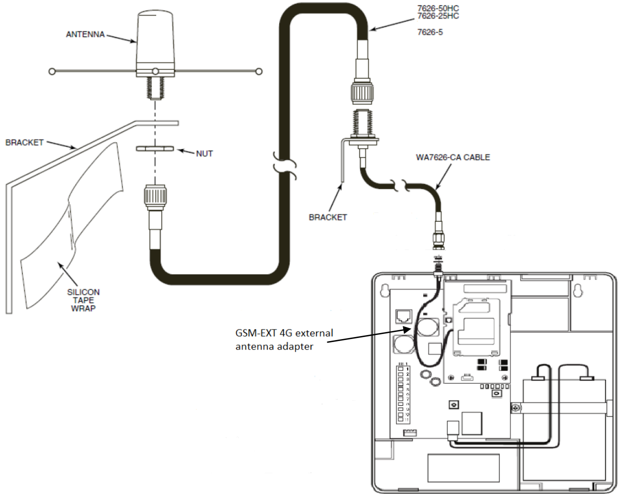
Illustration of a complete 3dB antenna install with all required components labeled
